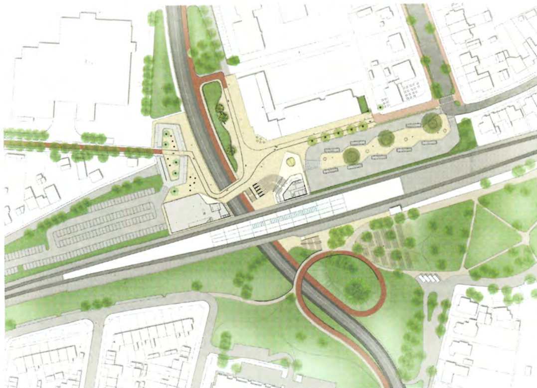
/ Design for the station area. On the northern side of the railway lines, the new station forecourt and concourse; on the southern side the coiled foot- and cyclepath that connects the station with the town centre.
